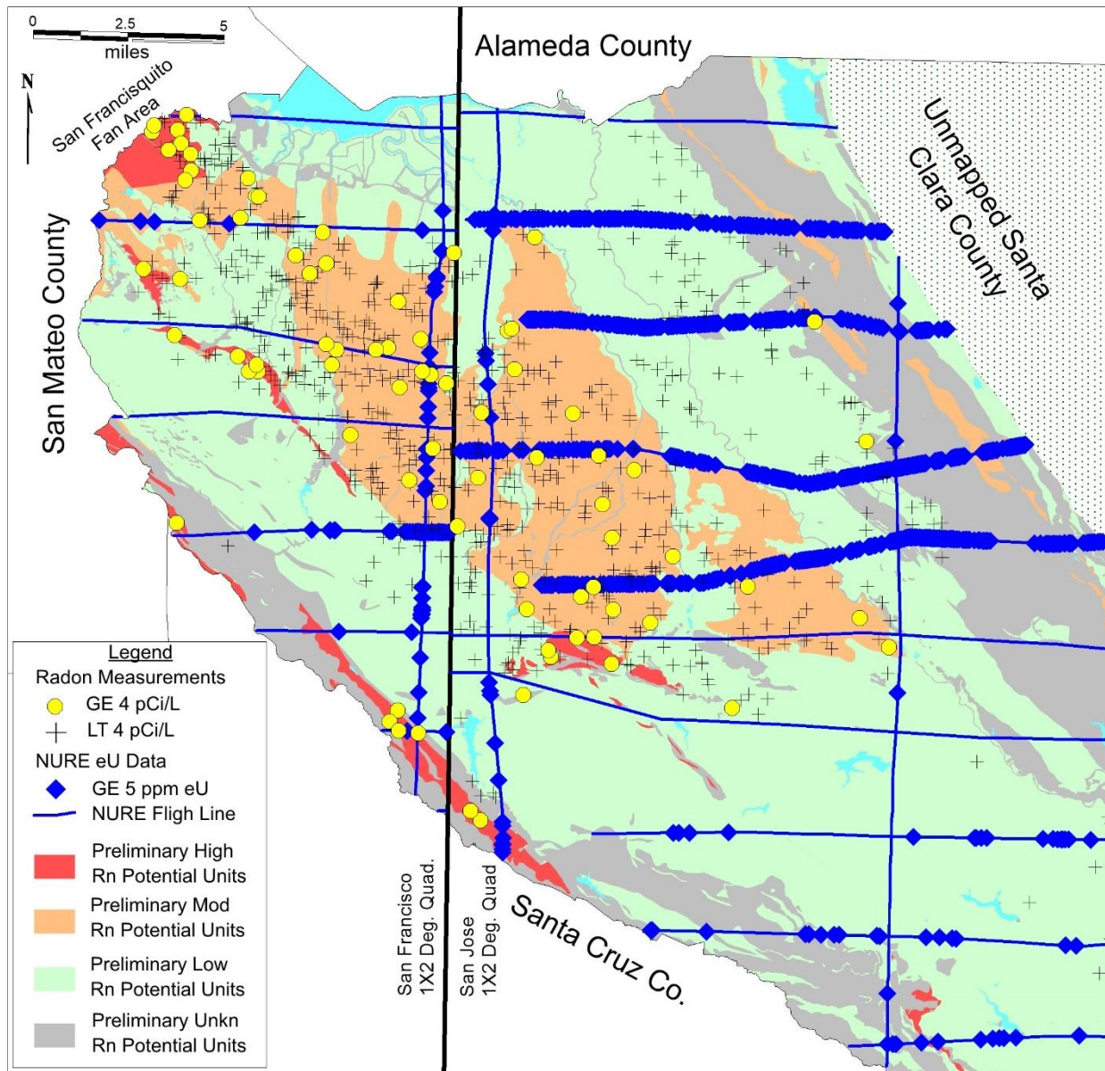
Figure H3. NURE eU data, CDPH radon survey data, and preliminary geologic unit radon potential areas
