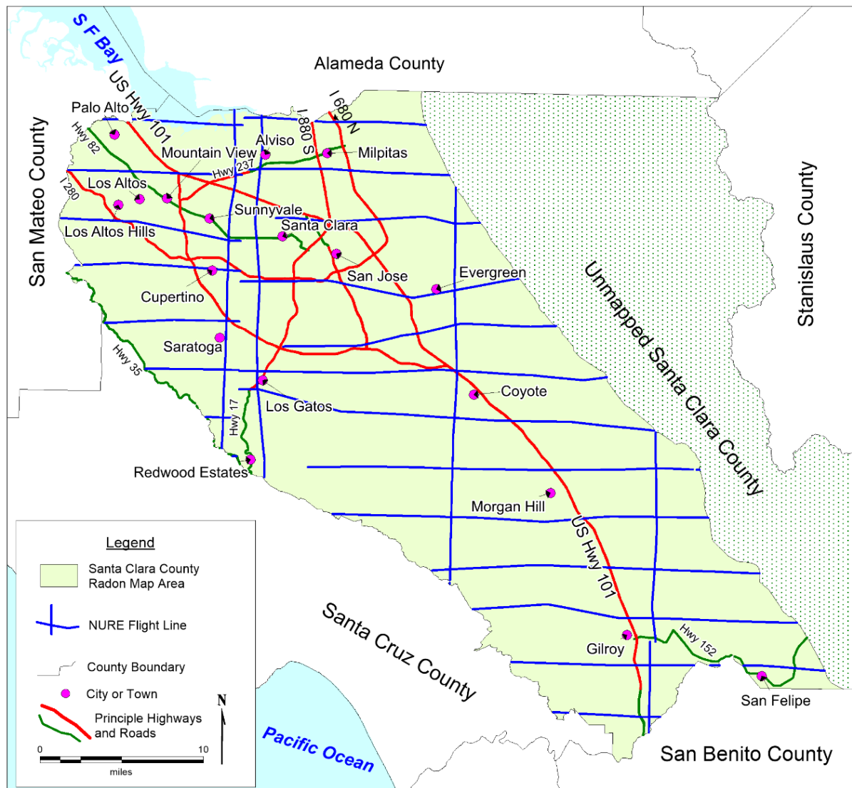
Figure H1. NURE program flight lines for Santa Clara County
