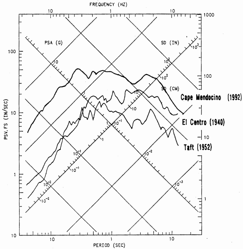
Figure 2. The 5% damped response spectra from the Cape Mendocino station (1992 Cape Mendocino mainshock), and for comparison, from Taft (1952 Kern County earthquake) and El Centro (1940 Imperial Valley earthquake) (figure from Darragh and others, 1993a).
