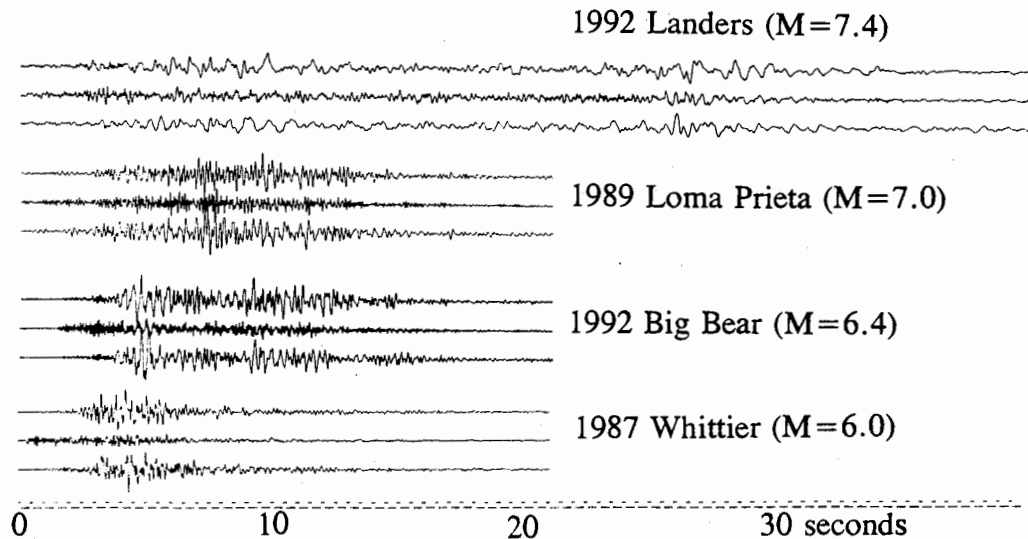
Figure 3. Accelerograms recorded for 4 different magnitude earthquakes at stations with similar distances (10 - 20 km). The waveforms demonstrate the long duration of the Landers earthquake (figure from Darragh and others, 1993a).
