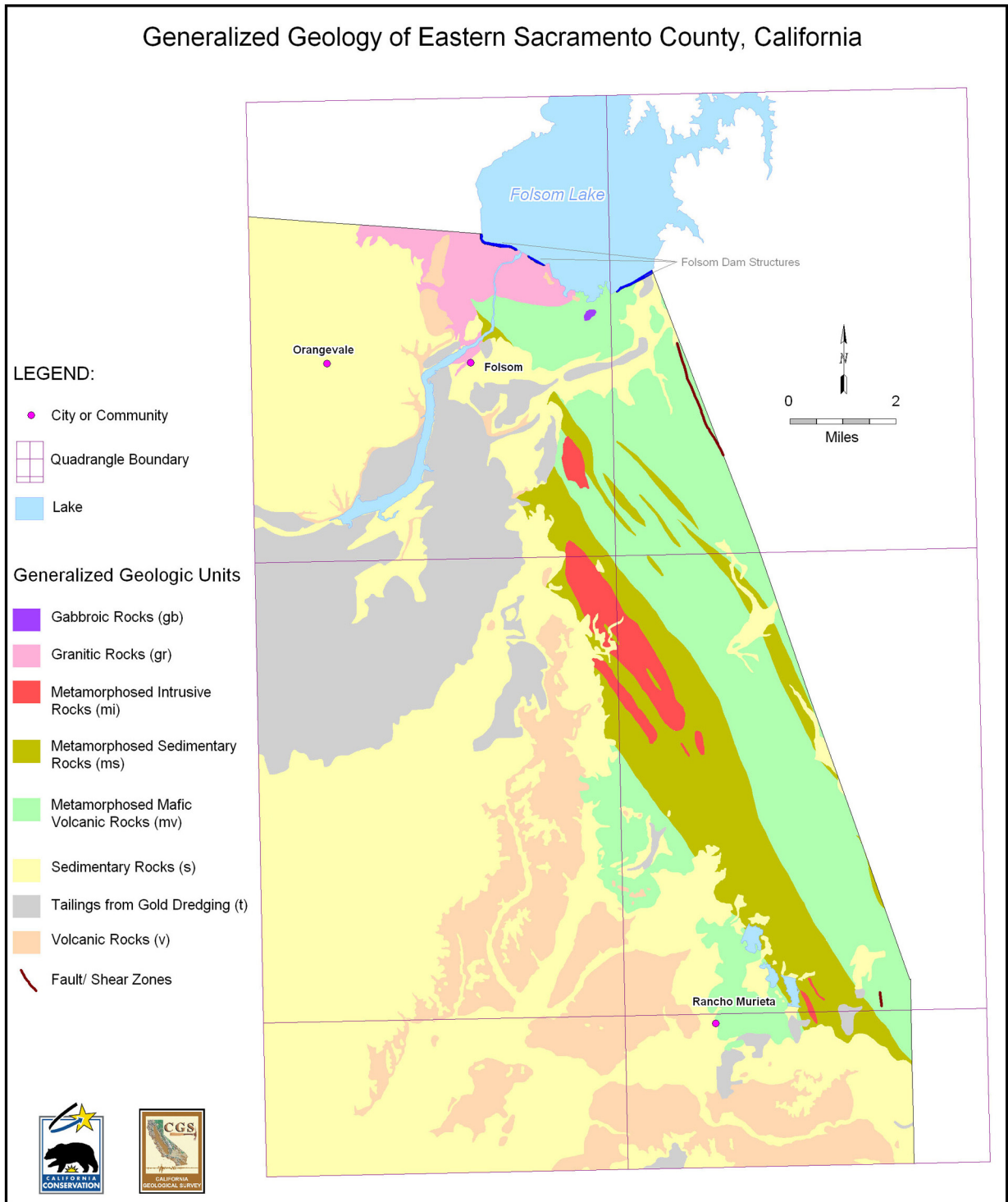
Figure 2. Generalized Geologic Map of Eastern Sacramento County.
